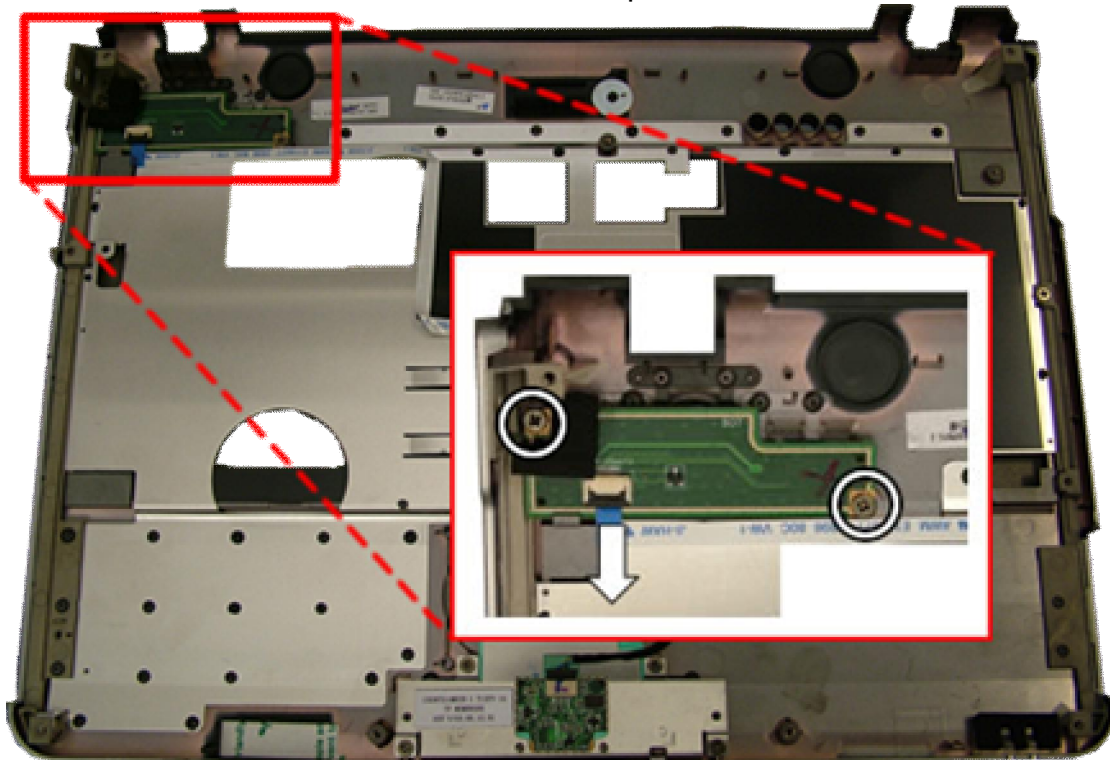
Fig. 20 The launch board.
